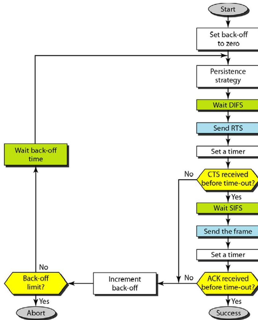
Figure 14.4 CSMA/CA flowchart
